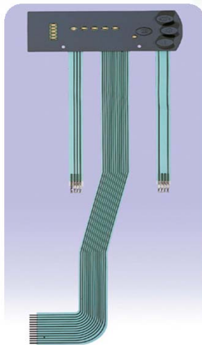
Membrane Touch Switches (MTS)
